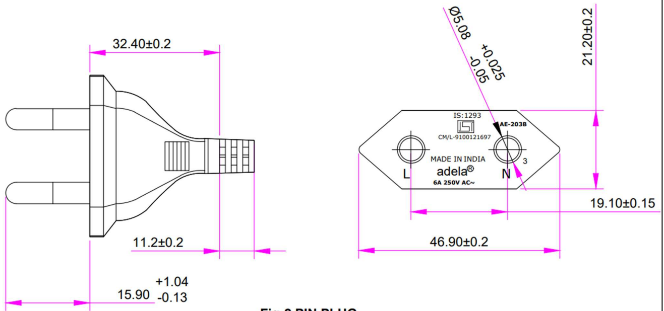
Fig-2 PIN PLUG
