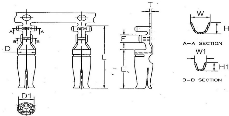
FIG : Various O Type Terminals
