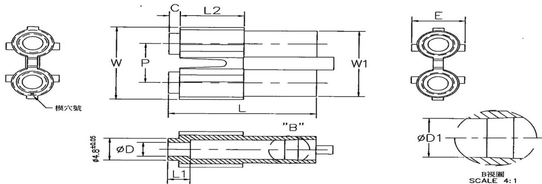
FIG : \phi 2.35 Housing
